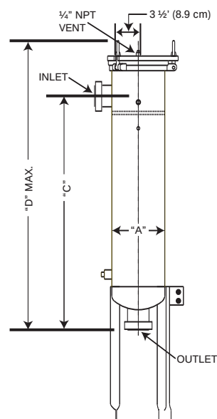
Side View (Flanged Housing)
