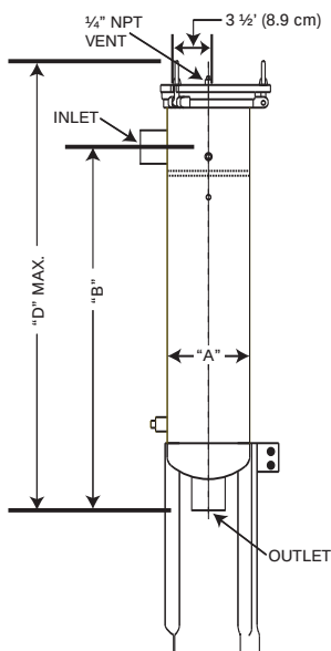
Side View (NPT Housing)
