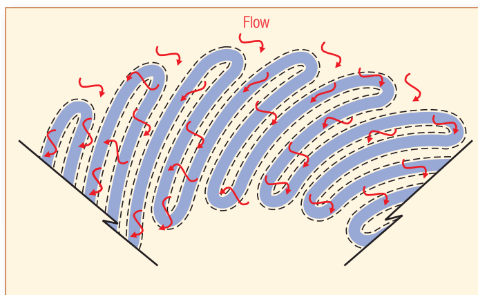
Figure 1: Uniform flow distribution of an Ultipeat filter
