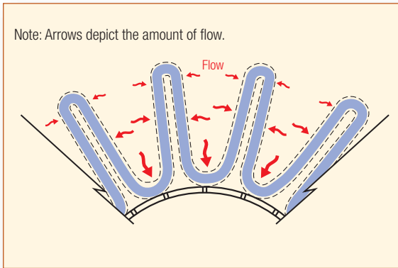
Figure 3: Non-uniform flow distribution in a traditional fan-pleat filter
