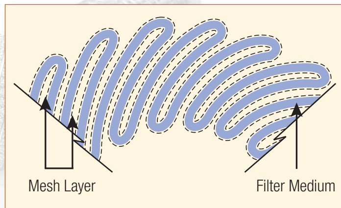
Figure 2: Ultipeat filter element construction
