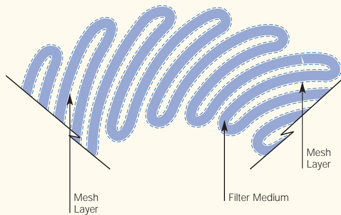
Figure 3. Ultipleat filter element construction
