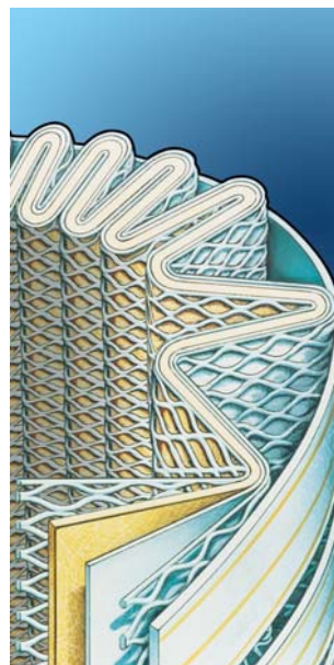
Ultipor® Plus filter element construction
