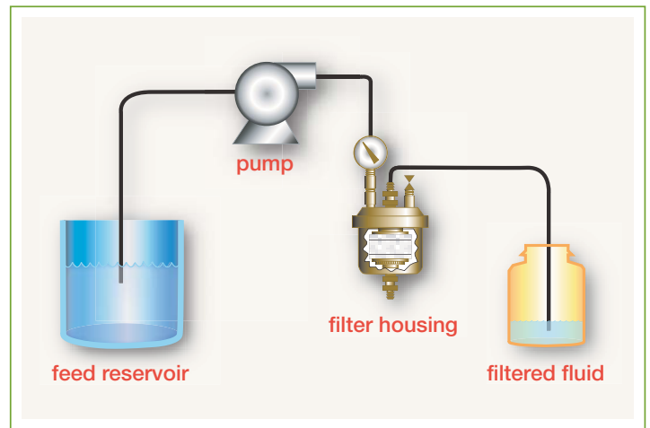
Figure 1: Equipment set-up for filterability testing
