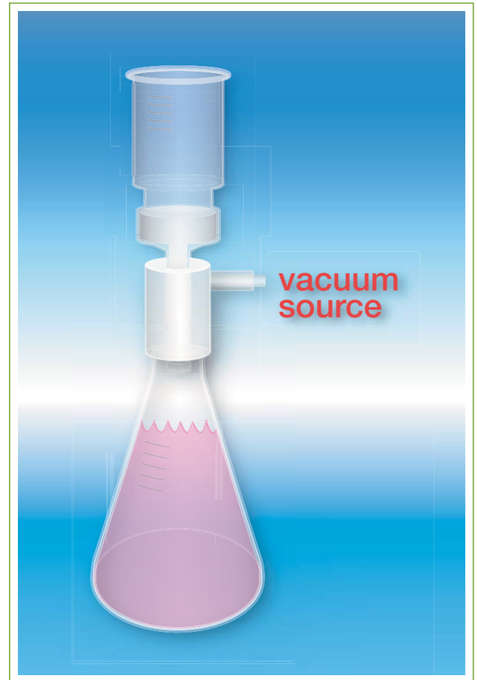
Figure 3: Equipment set-up for ink cleanliness quality testing
