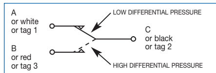
Figure 1a - Stainless Steel Switch Circuit Diagram
