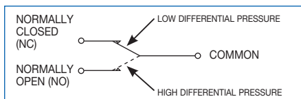
Figure 1 - Typical Switch Circuit Diagram for SPDT (Single Pole Double Throw) type switches.
