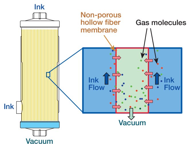
Figure 2: Schematic of fiber showing directional flow
