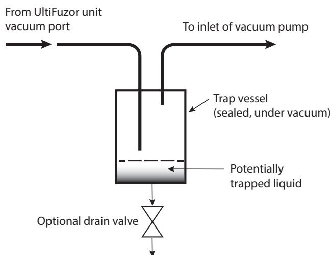
Figure 3: Schematic of a liquid trap set-up
