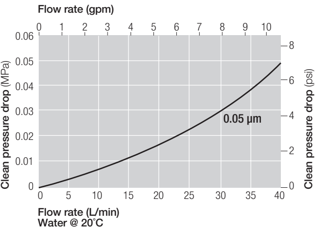
UltiKleen G2 KC Assembly (L-flow and T-flow, 3/4" nozzle)
