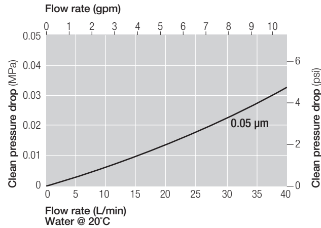
UltiKleen G2 Excellar KC Assembly (in-line, 1" nozzle)
