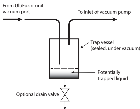
Figure 3: Schematic of a liquid trap set-up
