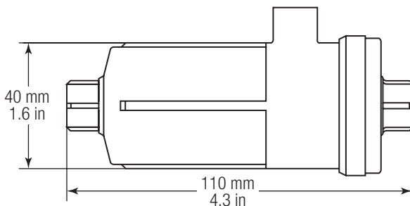
Figure 1: Dimensions
