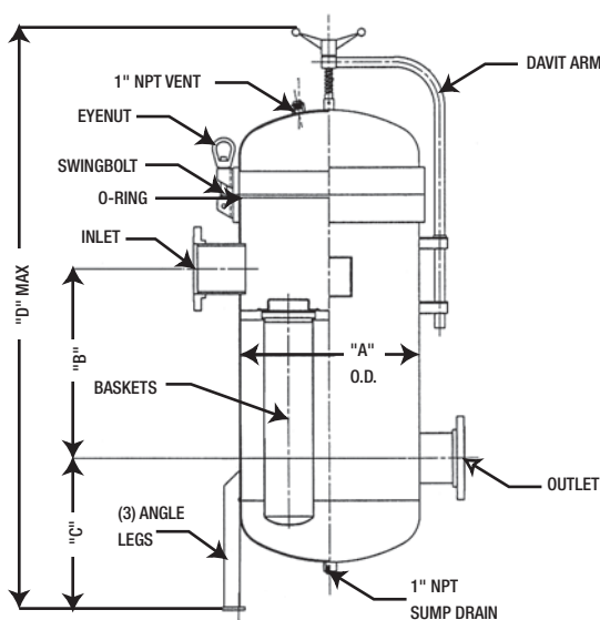
Side View (Multi-Around Housing)
