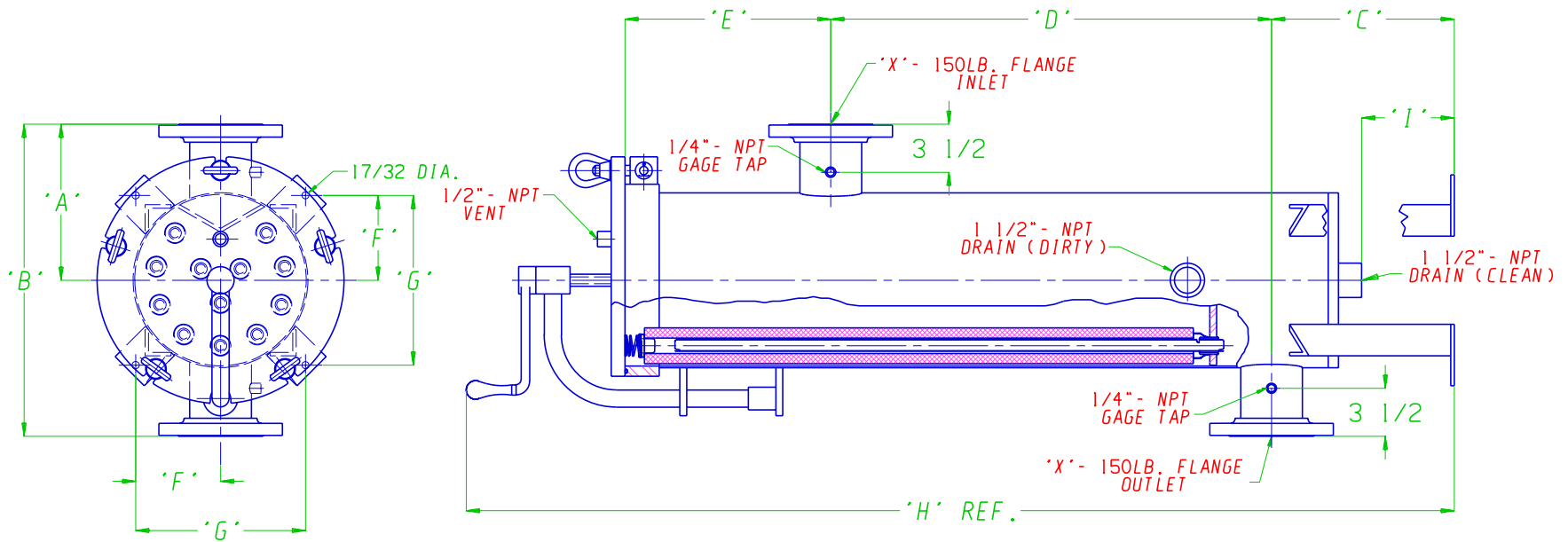
FSMC FILTER HOUSINGS STYLE 6 12 TO 27 CARTRIDGES A.S.M.E. CODE
