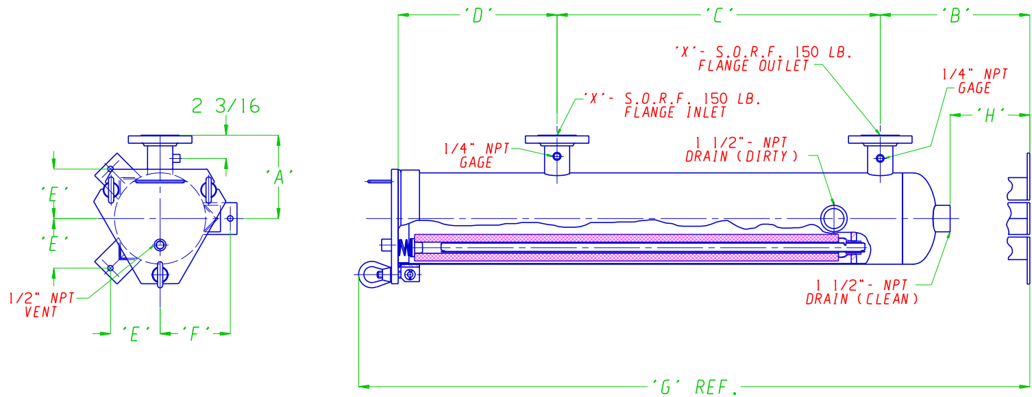
FSMC FILTER HOUSINGS STYLE 8 3 AND 6 CARTRIDGES A.S.M.E. CODE
